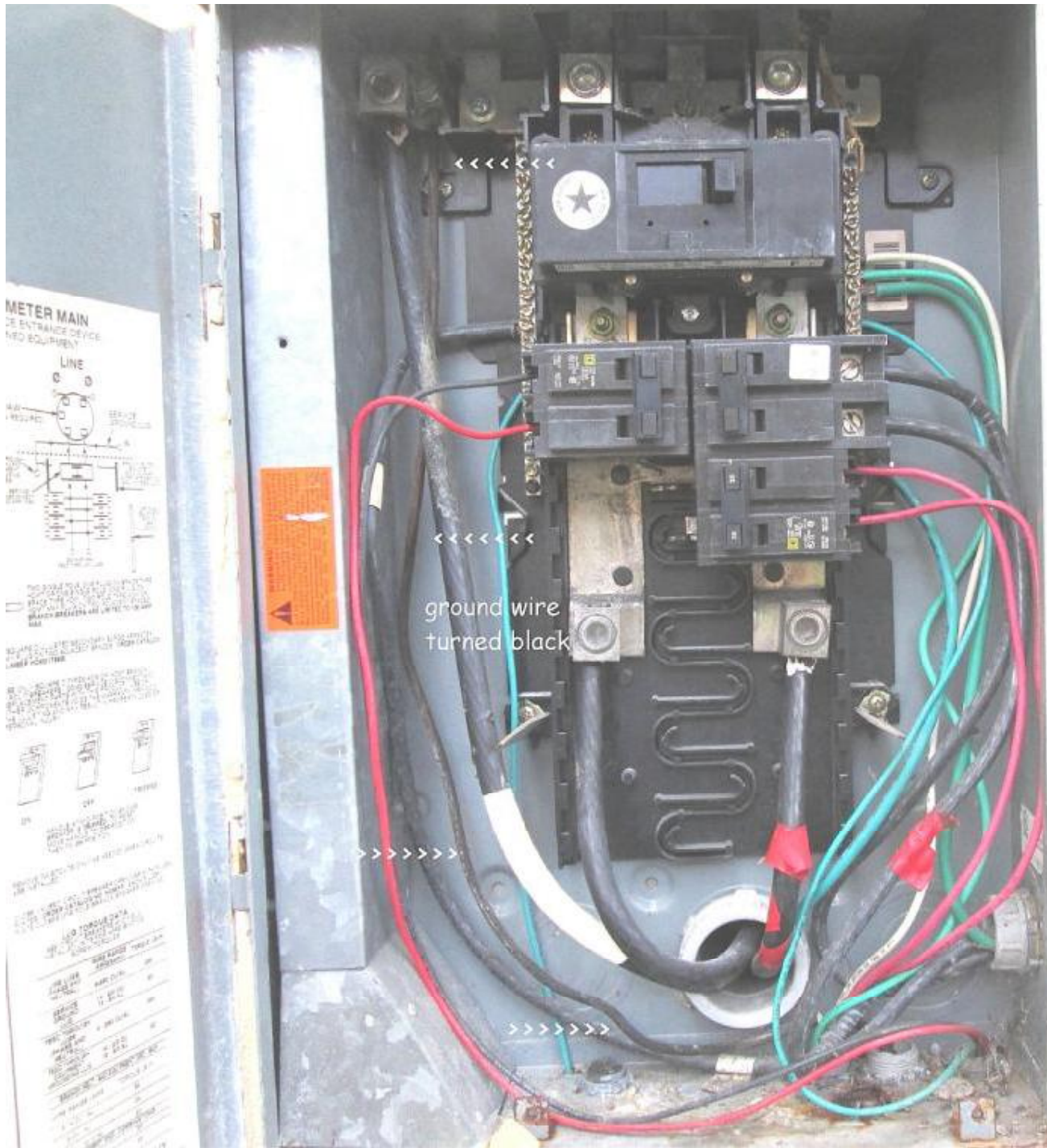
exterior circuit breaker panel on north side-200 amp service
